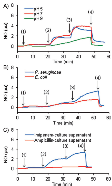
Figure 2. Amperometric characterization of NO release from 7 . A) NO release in the presence of penicillinase at varying pH values. Arrows indicate addition of the following to a reaction vial at 25°C containing 10 mL tris buffer at pH 9.0, 7.0, or 5.0: 1) 10 \mu L of 100 mM 7 , 2) 5 \mu L of 0.1 U \mu L^{-1} penicillinase, 3) 10 \mu L of 0.1 U \mu L^{-1} penicillinase, 4) 80 \mu L of 10 mM PTIO. B) NO release in the presence of cell extracts of P. aeruginosa pretreated with 50 \mu g mL^{-1} ampicillin or non- \beta -lactamase-expressing E. coli . Arrows indicate addition of the following to a reaction vial containing 10 mL tris buffer at pH 7.0: 1) 10 \mu L of 100 mM 7 , 2) 100 \mu L cell extract, 3) 200 \mu L cell extract, 4) 80 \mu L of 10 mM PTIO. C) NO release in the presence of supernatants from P. aeruginosa cultures grown for 5 h in the absence of antibiotic then treated for 1 h with imipenem (0.5 \mu g mL^{-1} ) or ampicillin (100 \mu g mL^{-1} ). Arrows indicate addition of the following to a reaction vial containing 10 mL tris buffer at pH 7.0: 1) 10 \mu L of 100 mM 7 , 2) 500 \mu L supernatant, 3) 500 \mu L supernatant, 4) 80 \mu L of 10 mM PTIO.
