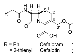
Figure 1. Chemical formulas of cephalosporin antibiotics, Cefaloram 1 and Cefalotin 2 .
