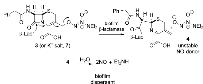
Scheme 1. Proposed mechanism of \beta -lactamase-triggered NO release and biofilm dispersion by cephalosporin-3'-diazoniumdiolate 3/7 .
